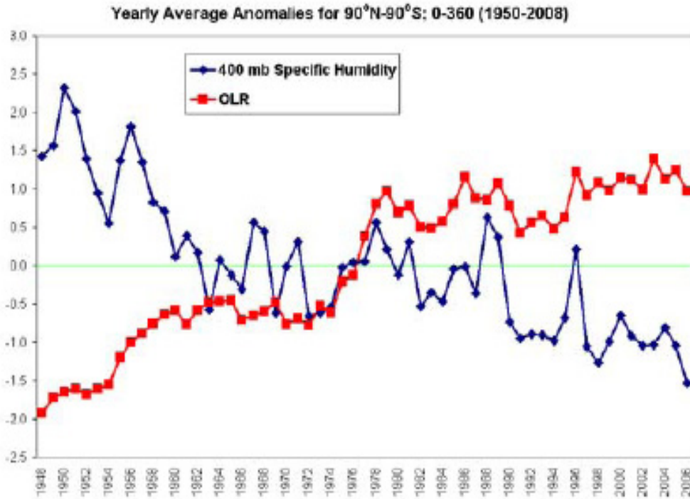
Figure 6. NCEP/NCAR reanalysis of standardized anomalies of 400 mb (~7.5 km altitude) water vapor content (i.e. specific humidity – in blue) and Outgoing Longwave Radiation (OLR) from 1950-2008. Note the downward trend in moisture and the upward trend in OLR.
